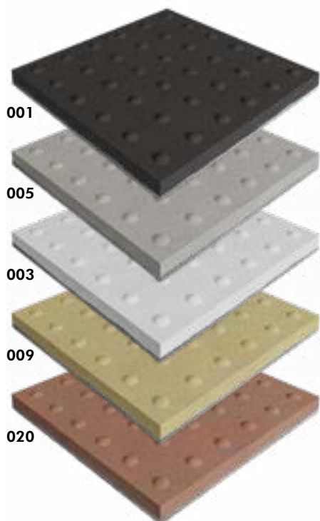
PAVIMENTO DE PERIGO (ALERTA) ALC011752 BLISTER SURFACE TACTILE PAVING 40x40x3 cm ≈ 69 Kg/m 2
