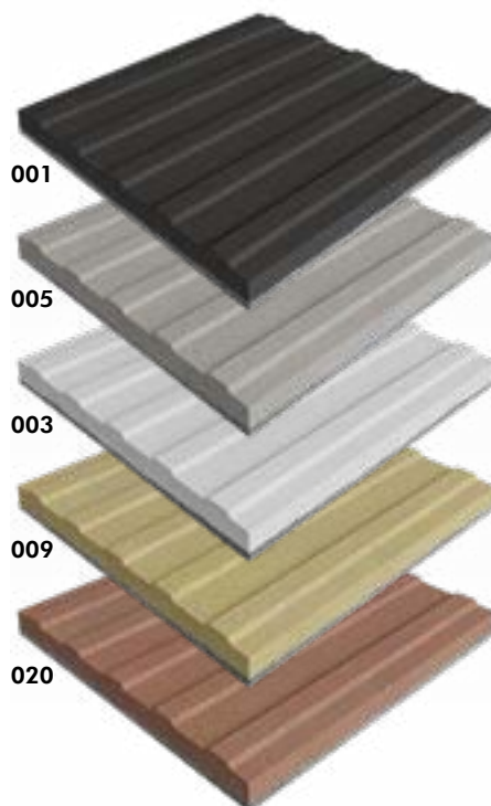
PAVIMENTO DIRECIONAL (GUIA) ALC011753 DIRECTIONAL GUIDANCE SURFACE PAVING 40x40x3 cm ≈ 69 Kg/m 2
